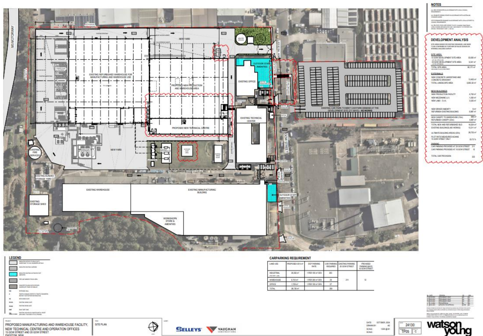
Figure 1: Site Plan/Warehouse Ground Floor
